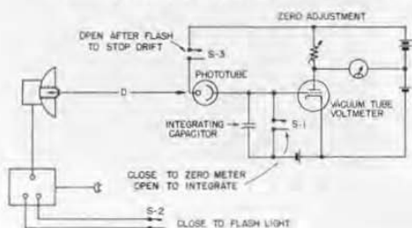
Figure 2. Elementary schematic of the electrical circuit.
