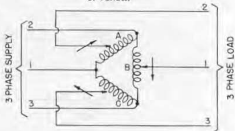
Figure 1. Circuit for closed delta connection of Variacs.
